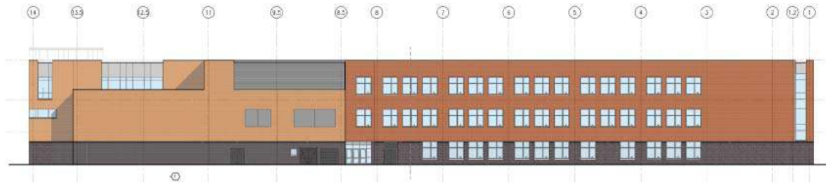
2 WEST ELEVATION 1/8" = 1'-0"
