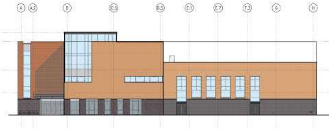
2 NORTH ELEVATION 1/16" = 1'-0"
