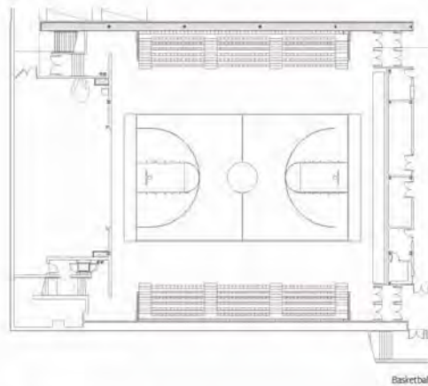
Basketball Seating Layout Bleachers (Fully Deployed) 7 rows @ 12" rise 26" row spacing 300 seats each side (600 total)
