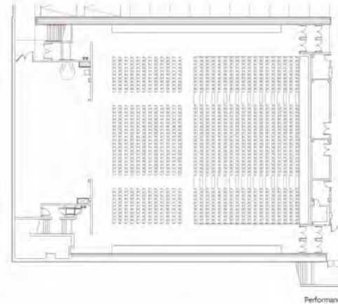
Performance Seating Layout Telescoping Seating 6 rows @ 12" rise 36" row spacing 150 + 450 in-use = 1500 seats total
