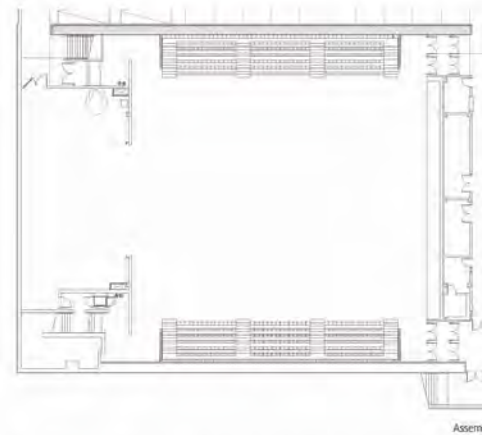
Assembly Seating Layout Bleachers (Fully Deployed) 7 rows @ 12" rise 26" row spacing 300 seats each side (600 total)
