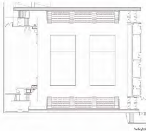
Volleyball Seating Layout Bleachers (Fully Deployed) 7 rows @ 12" rise 26" row spacing 300 seats each side (600 total)
