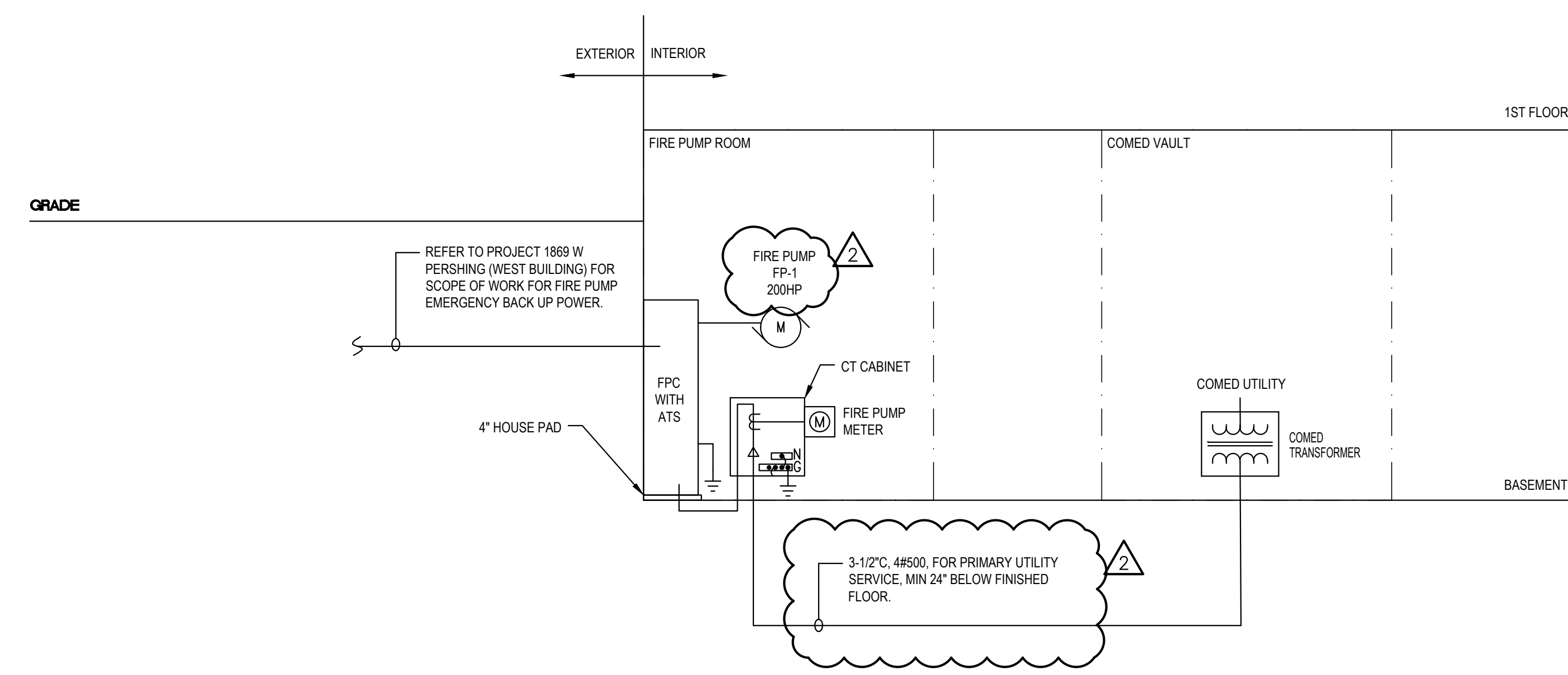
2 FIRE PUMP SERVICE SINGLE LINE DIAGRAM NOT TO SCALE
