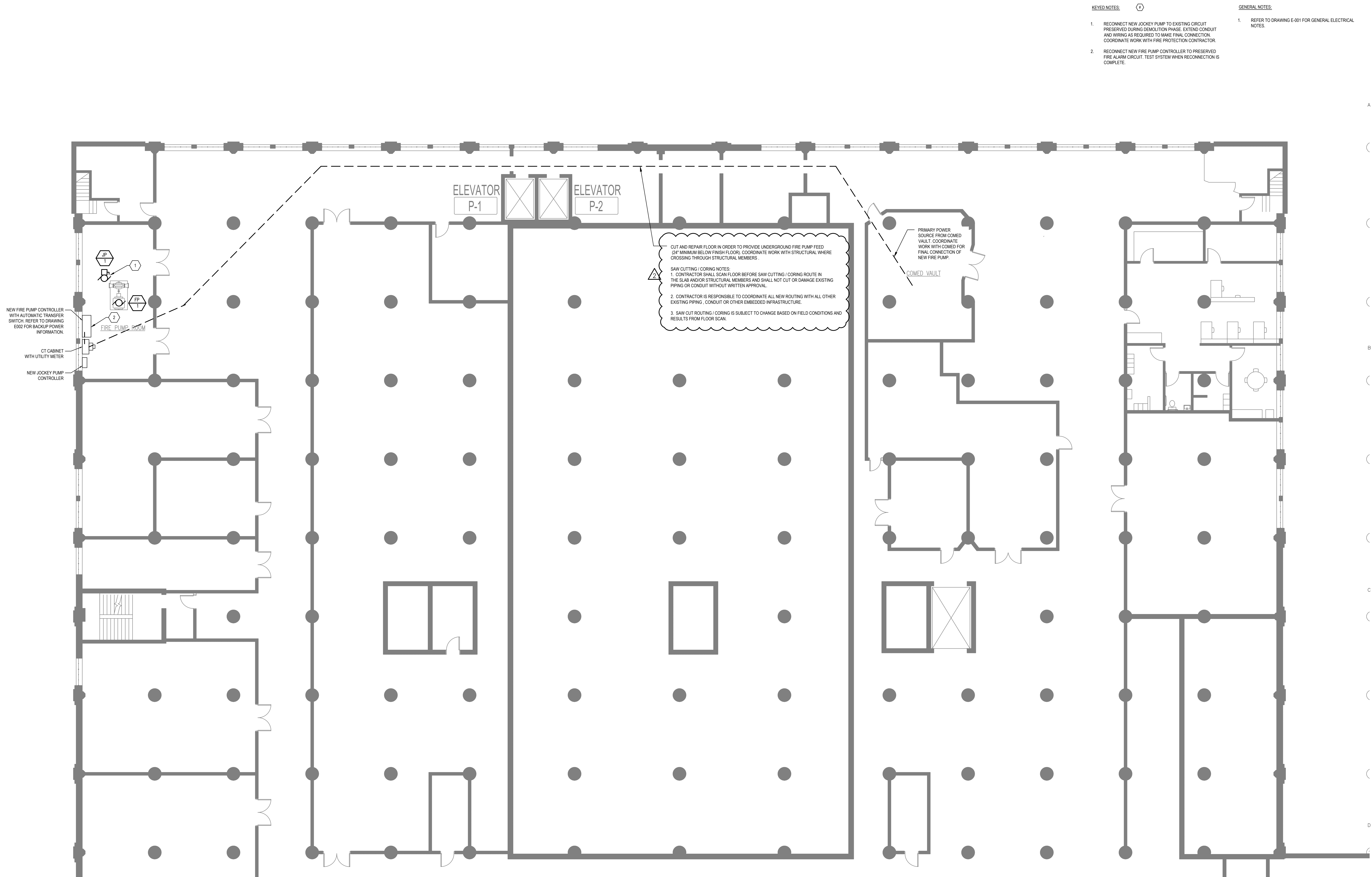
1 BASEMENT ELECTRICAL POWER PLAN - NORTH - WEST BLDG SCALE: 1/8"=1'-0"
